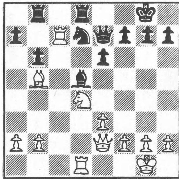
489 After 20...Nd7
